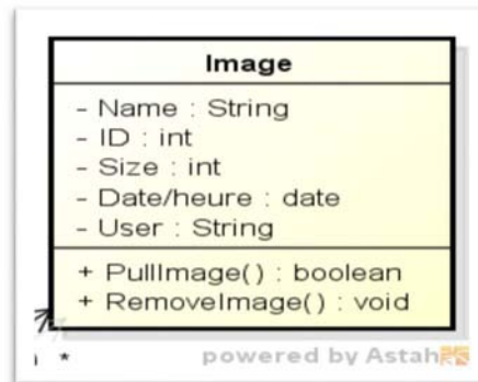
Figure 21 : Classe Image
