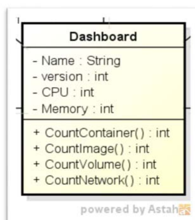
Figure 25 : Classe Dashboard
