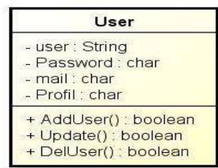
Figure 22 : Classe User
