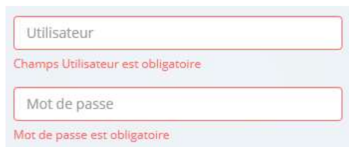
Figure 42 : Bootstrap Validator
