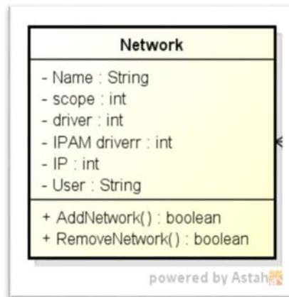
Figure 24 : Classe Network
