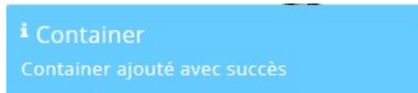
Figure 41 : Bootstrap Notify
