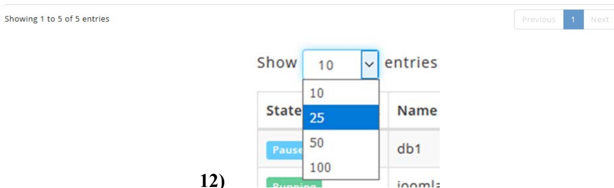
Figure 46 : Data Tables
