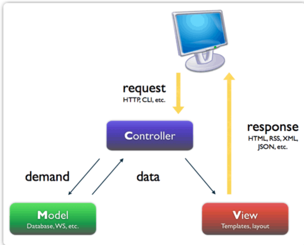
Figure 11: Architecture MVC [7]
