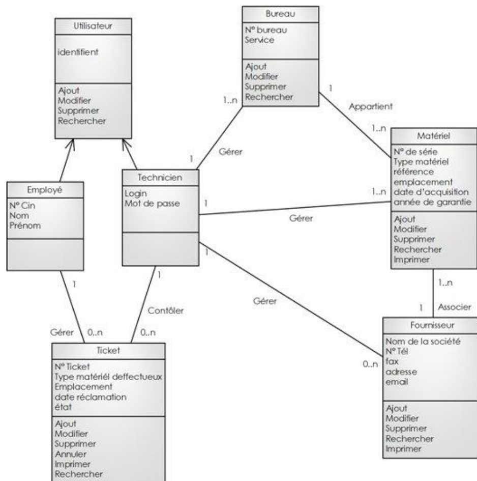
Figure 10: Diagramme des classes
