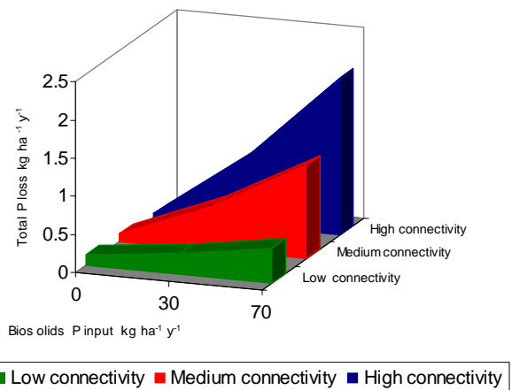
Fig. 11. Predicted loss assuming changes in biosolid application rates and hydrological connectivity
