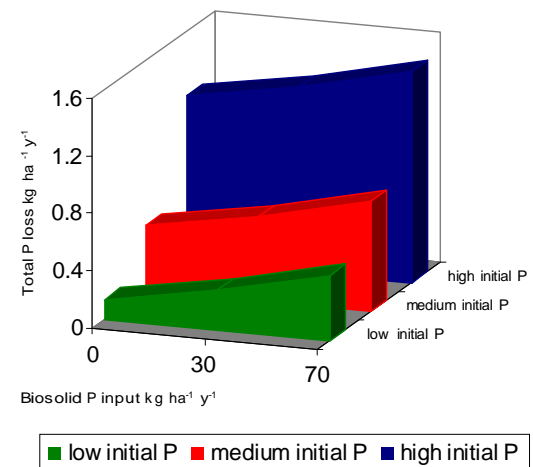
Fig. 12. Loss under conditions of low connectivity but with a range of initial soil conditions reflecting the history of applications in a catchment
