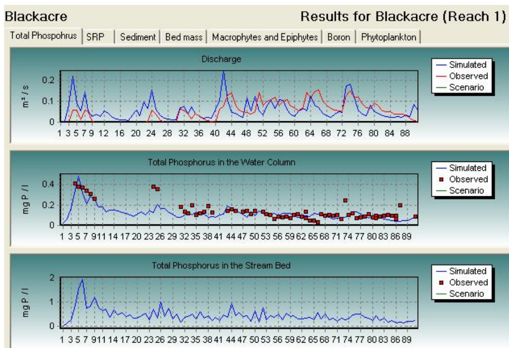
Fig. 8. Simulation of flow, SRP and total phosphorus for the Blackacre field site over 90 days from 01 November 2003
