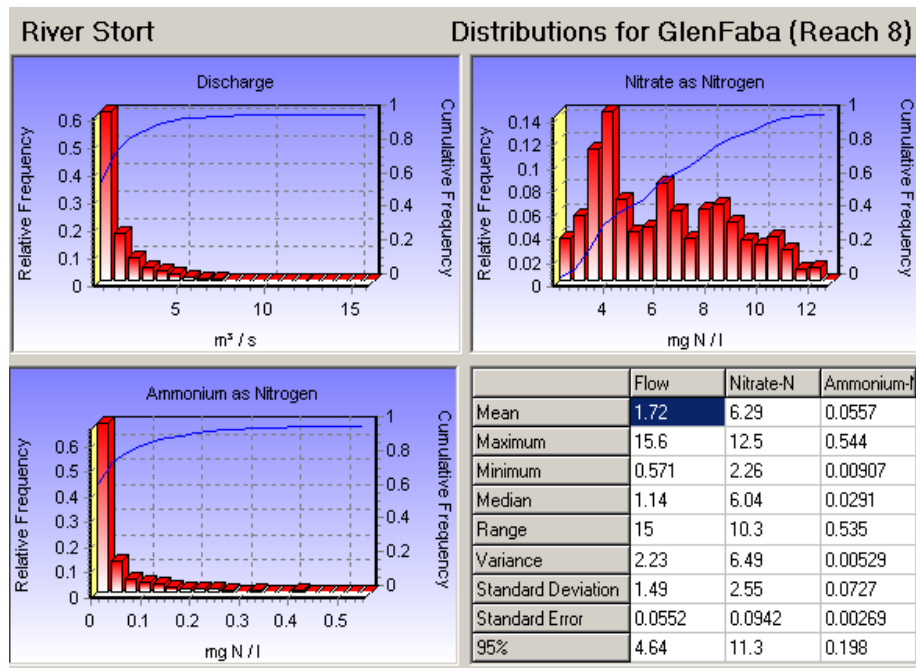
Fig. 6. Distributions of flow, nitrate and ammonium at Glen Faba on the Start
