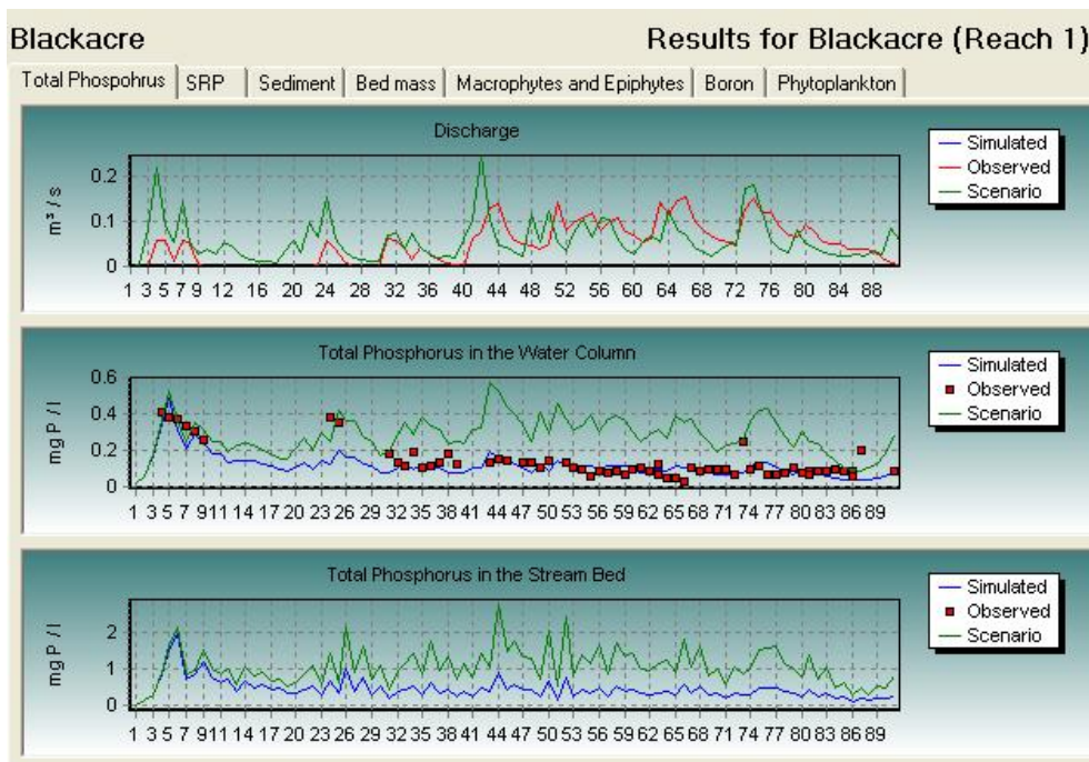
Fig. g. Simulation of flow SR and total for the Blackacre field site over 90 days from 0 November 003 assuming an additional application of biosolid.
