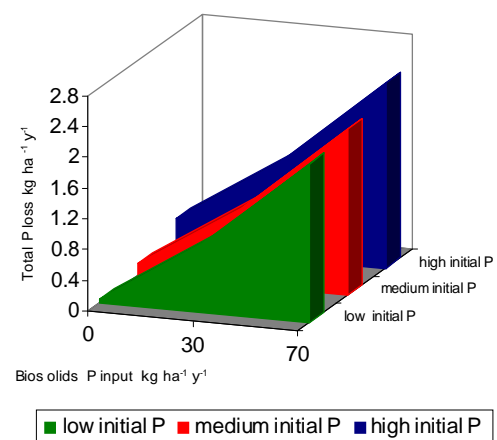
Fig. 13. Loss for a system that has high connectivity but with a range of initial soil conditions reflecting the history of applications in a catchment
