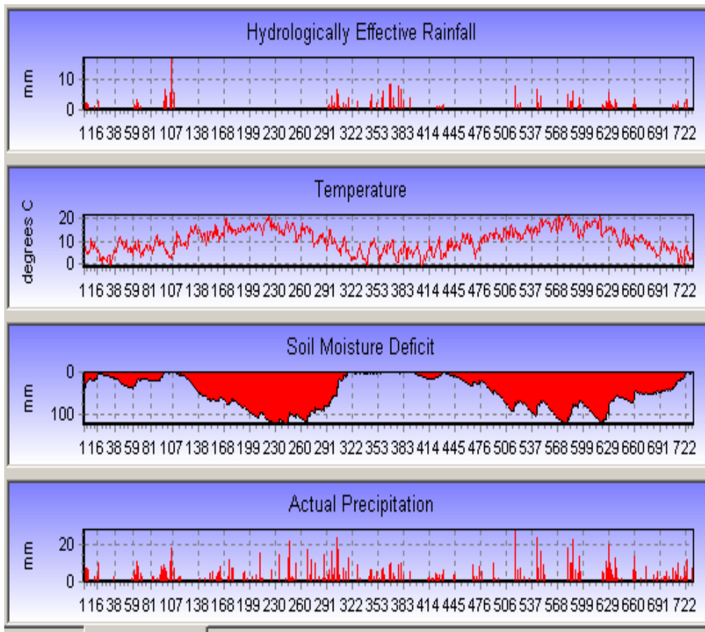
Fig. 3. Input daily time series for the River Stort for the year 1998 and 1999
