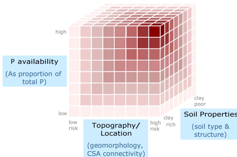
Fig. 10. The Nutrient Export Risk Matrix - the NERM - used to evaluate the availability of from agricultural land to water according to the key indicators of nutrient loss, namely soil properties and topography.
