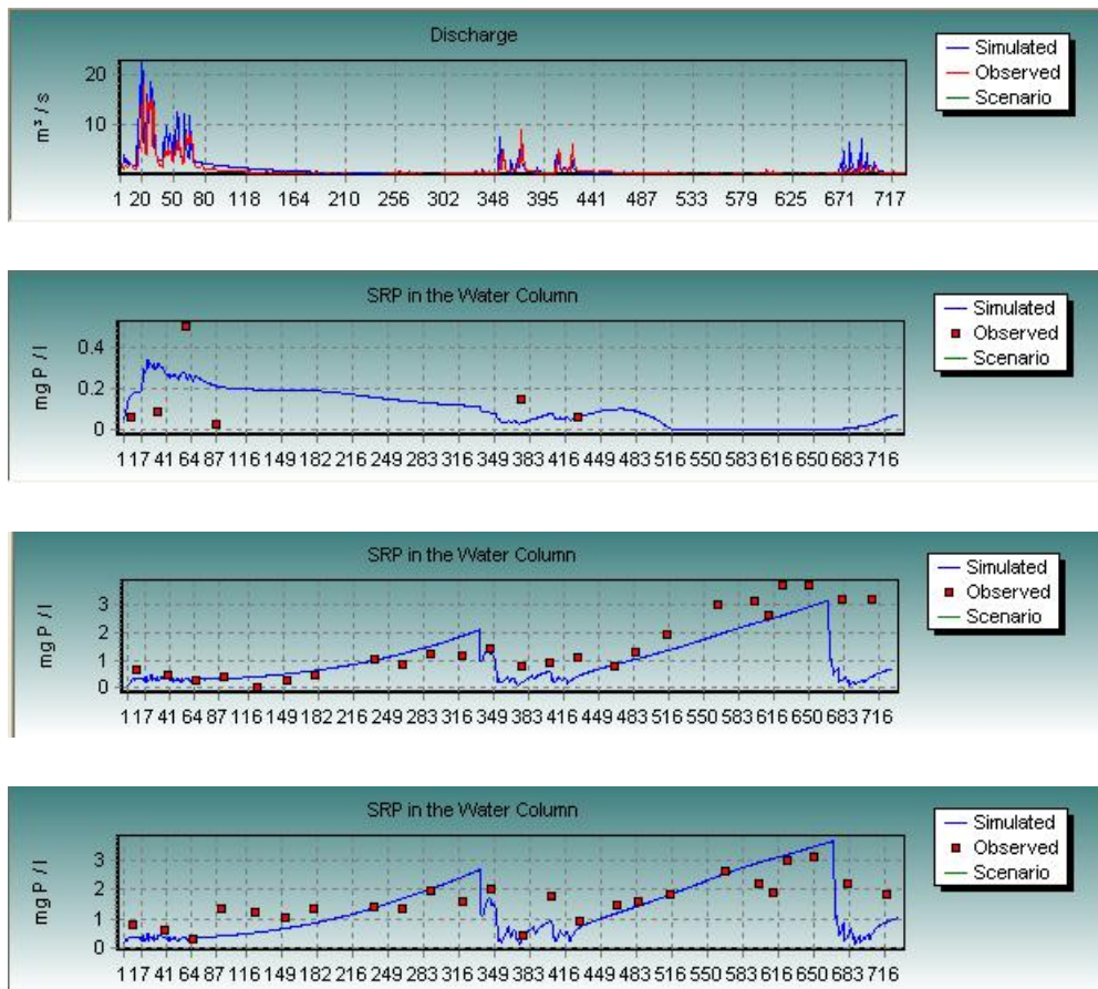
Fig. g. bserved and simulated response over 1999-1999 for the River Start at Glen Faba for flow and oor Bridge, Twyford Mill, Glen Faba for SR - observed data in red
