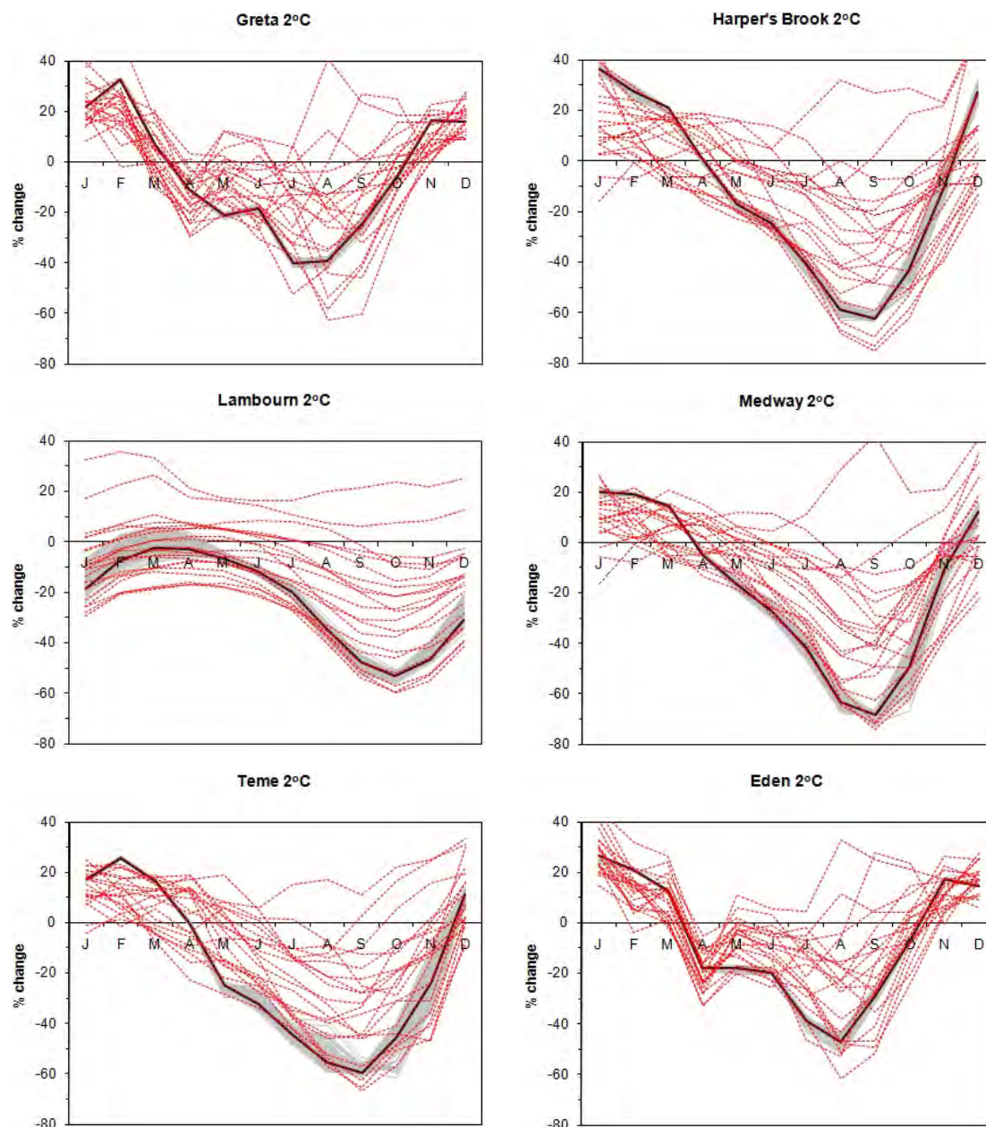
Fig. 8. Change in mean monthly runoff for the each catchment for a 2 °C rise in global mean temperature, under the 21 climate scenarios and, for the HadCM3 pattern, 100 sets of catchment model parameters.
