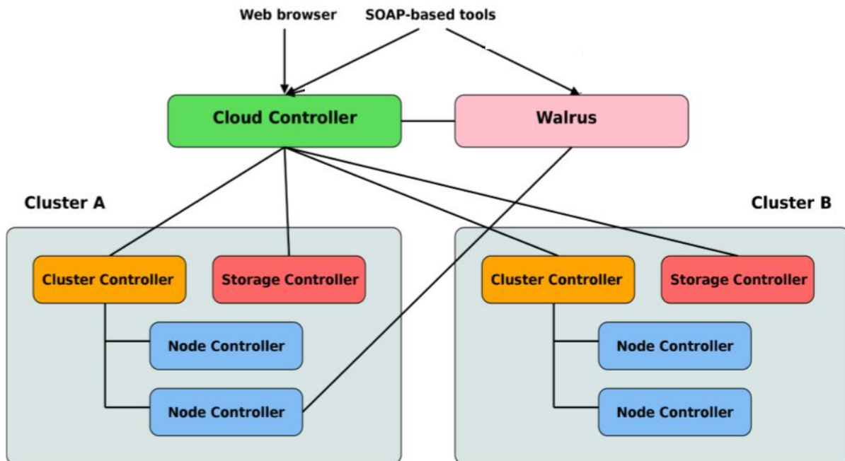
Figure 3.4-Structure architecturale d' Eucalyptus
