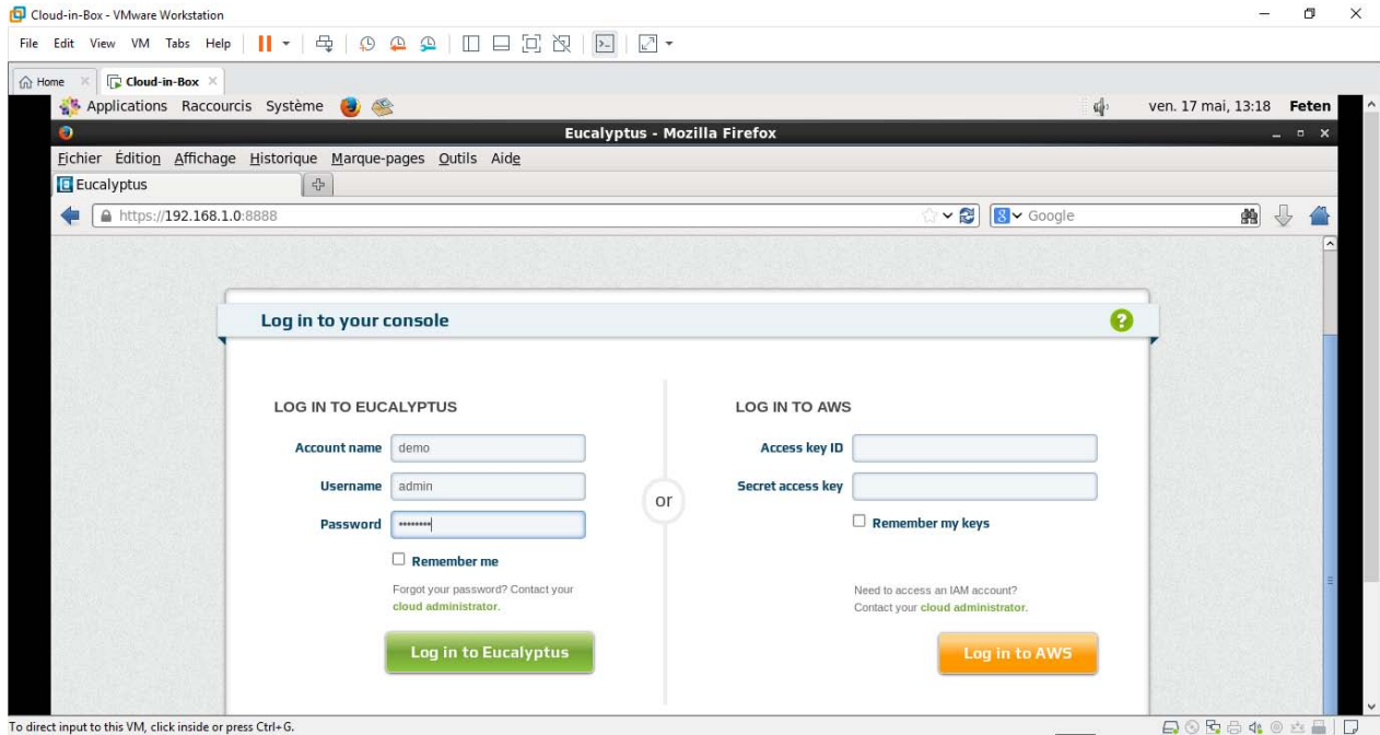
Figure 4.5-Interface Locataire
