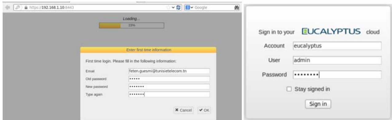
Figure 4.6-Interface Admin Cloud
