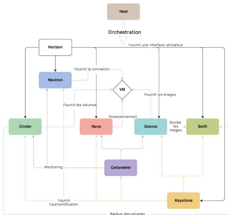
Figure 3.2-Architecture et composants d'OpenStack (ANEQ, 2018)
